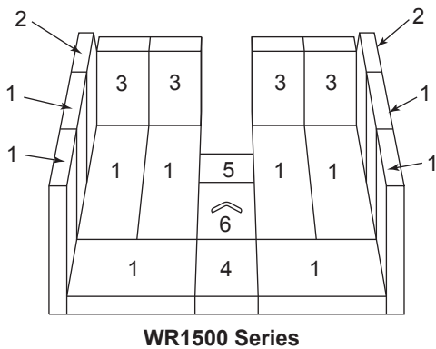
Figure 3 Fire Brick Installation
