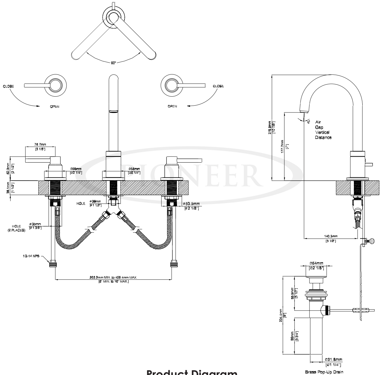
Product Diagram
