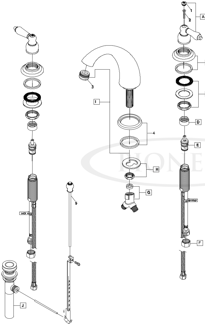
Product Diagram
