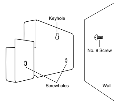
Figure 18: Mounting the Timer
