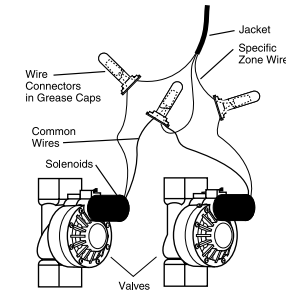
Figure 19: Wiring Valves
