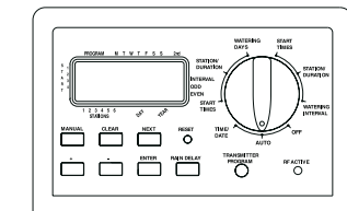
Figure 1: Location of Controls on the Timer
