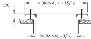
935 Square (Stamped Steel One Piece Frame)
