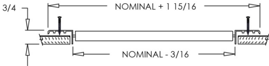
935 (Extruded Aluminum Frame)
