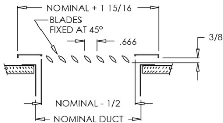
935 (Stamped Steel One Piece Frame)
