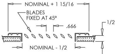
935 (Extruded Aluminum Frame)
