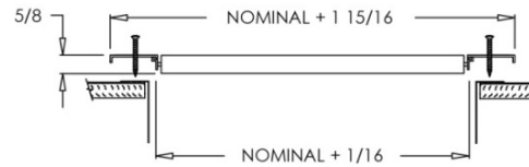
935 Rectangle (Stamped Steel One Piece Frame)
