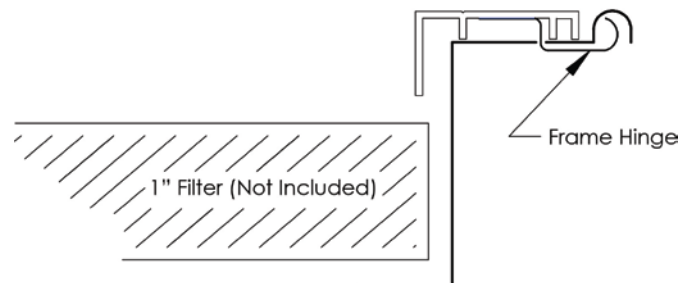
920FG1 Frame Detail
