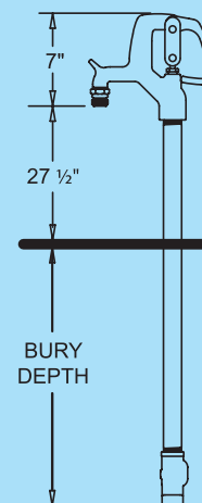
Rough-In Dimensions
