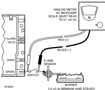
Fig. 7. S8700B,E,J,L single rod flame current measurement.
