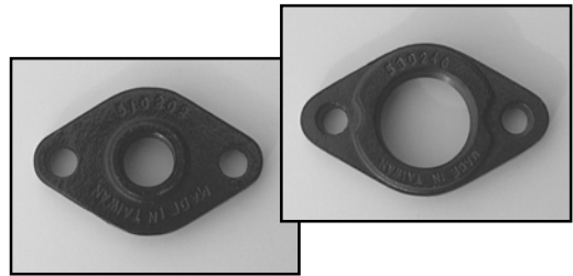
Cast Iron (Threaded) 3/4" = Part #519601 1" = Part #519602 1-1/4" = 519603 1-1/2" = 519604 (Special 1-1/2" for UP43-75F only) Part #539605
