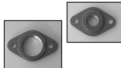
Bronze (Threaded) 3/4" = Part #539651 • 1" = Part #519652 (Special 1-1/2" for UP43-75BF) Part #539615
