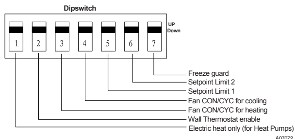
Configuration Switches
