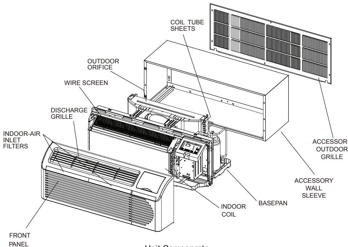
Unit Components
