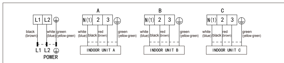
To the power supply
