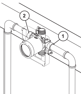
Iron Pipe
