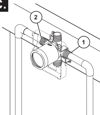
Copper Tubing
