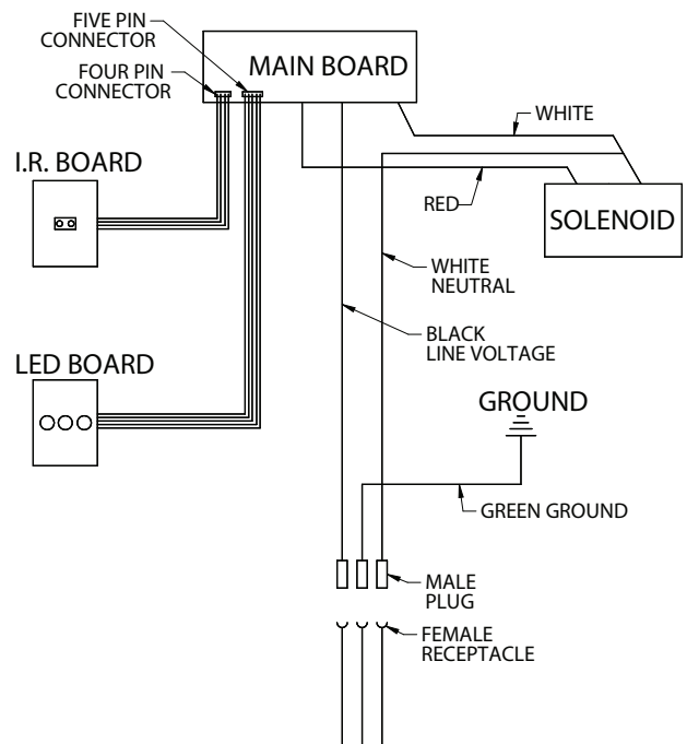
Electrical Diagram
