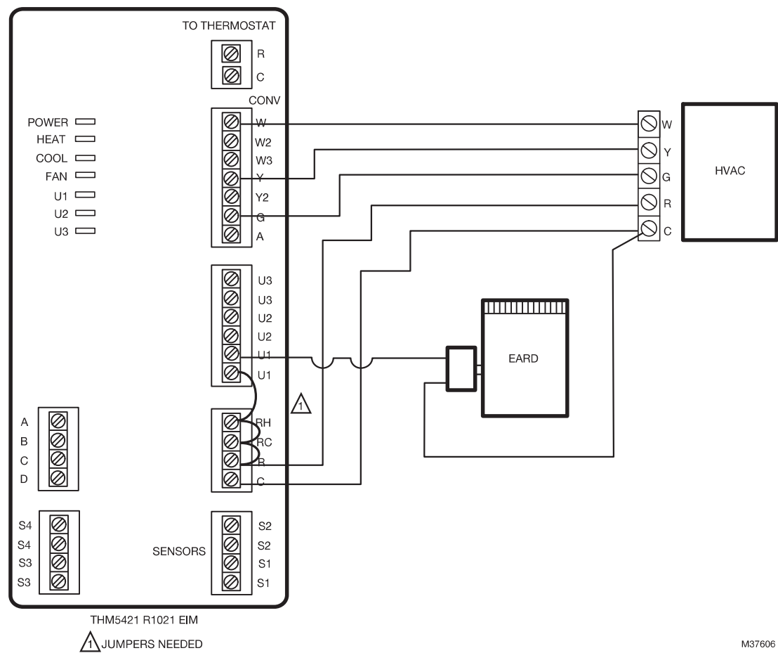
Fig. 5. TH8321R or Prestige with EIM controlling EARD damper.
