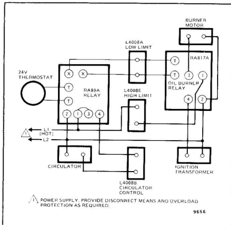
Fig. 5—Typical connection diagram for an oil-fired, hydronic heating system that provides year-round domestic hot water.
