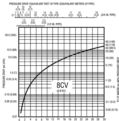
Fig 2c. Flow characteristics of 8 Cv (6.9 kV) valve.
