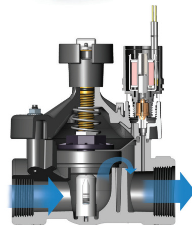
PESB Cutaway
